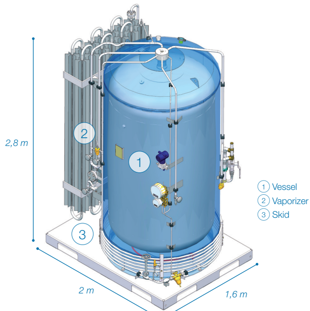
Skid Tank 3000 L 16 barg (PED compliant)
